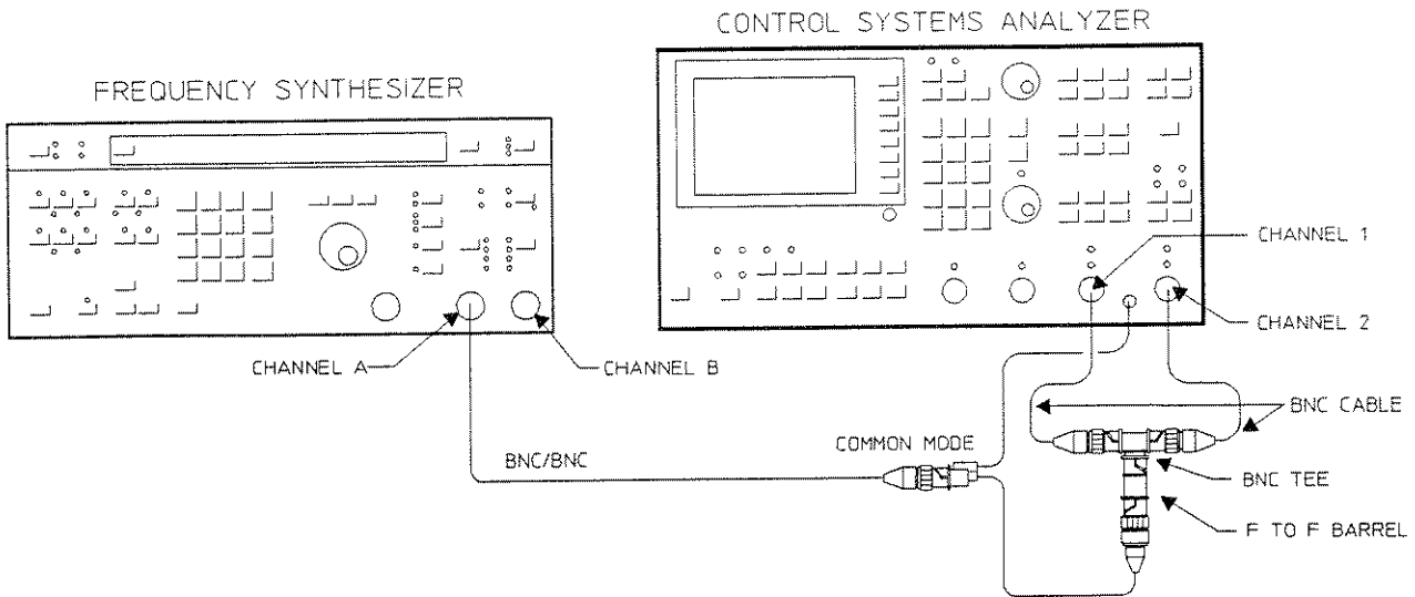
Figure 4-26. Common Mode Rejection Test Setup Two
